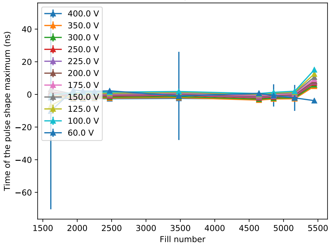
Time evolution of max. position for sector 2628
