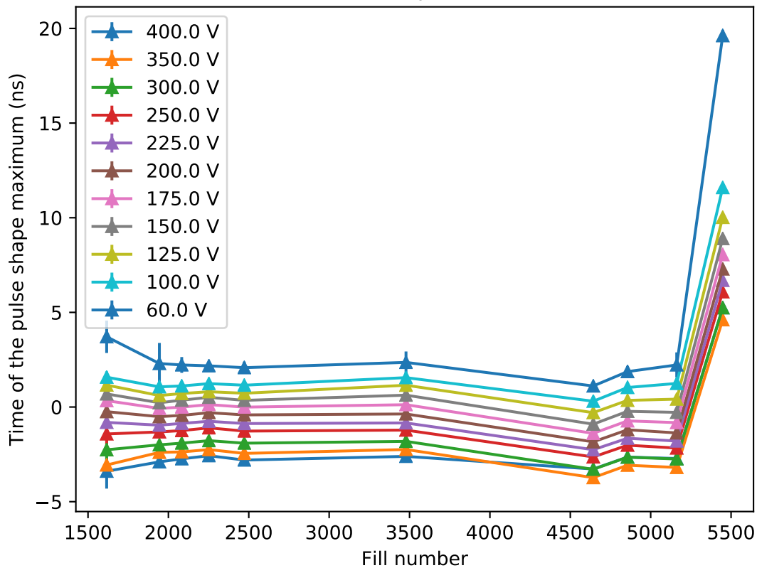
Time evolution of max. position for sector 2633
