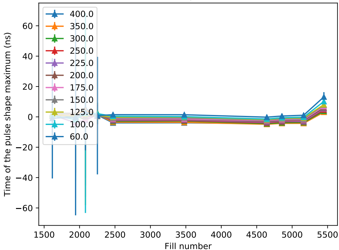
Time evolution of max. position for sector 2597
