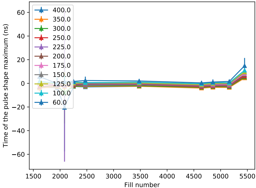
Time evolution of max. position for sector 2680
