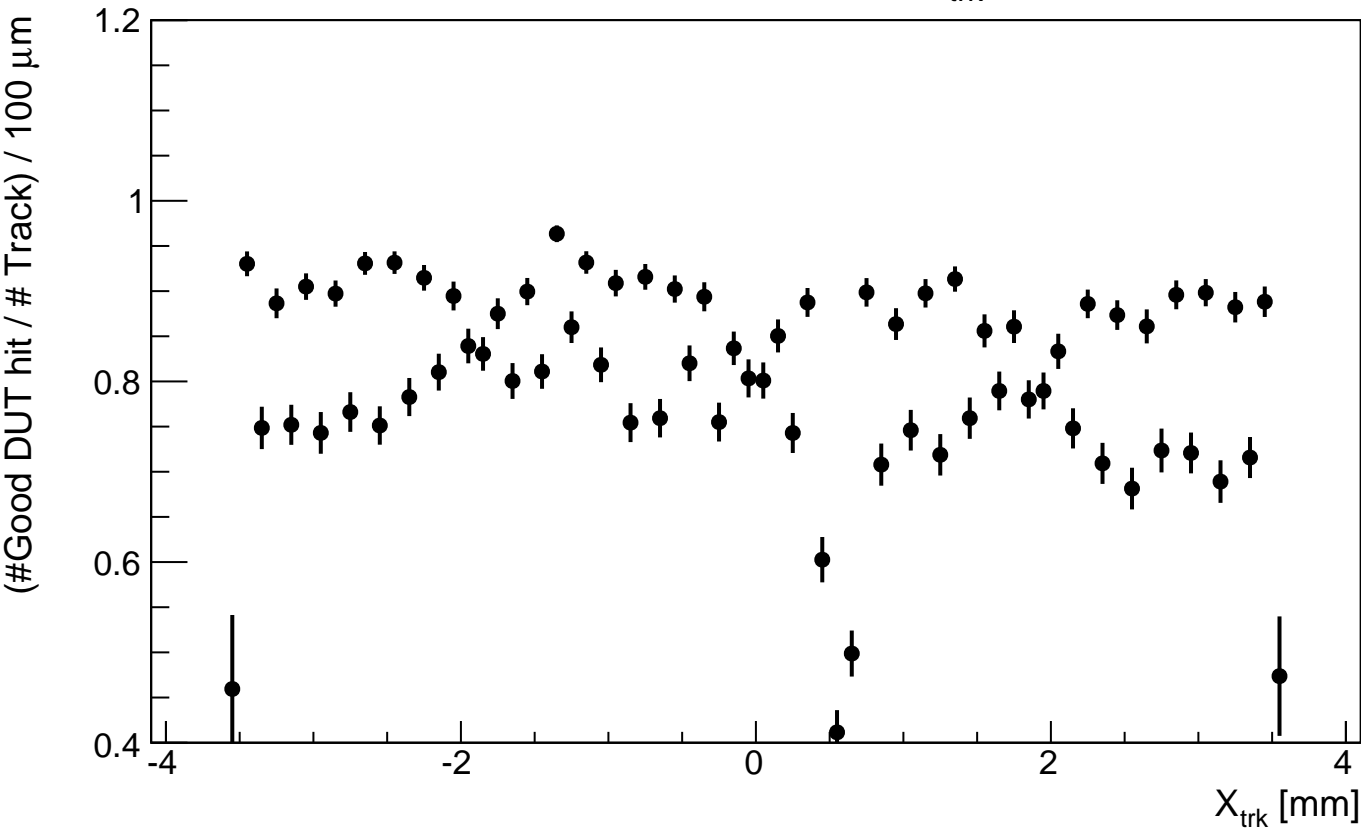
DUT Efficiency vs X_{\text{trk}}
