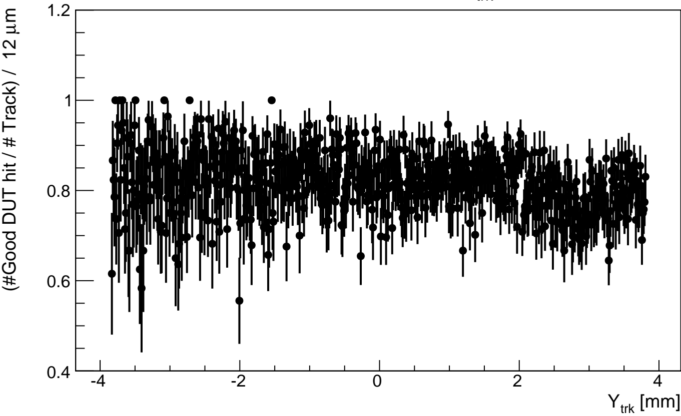
DUT Efficiency vs Y_{\text{trk}}
