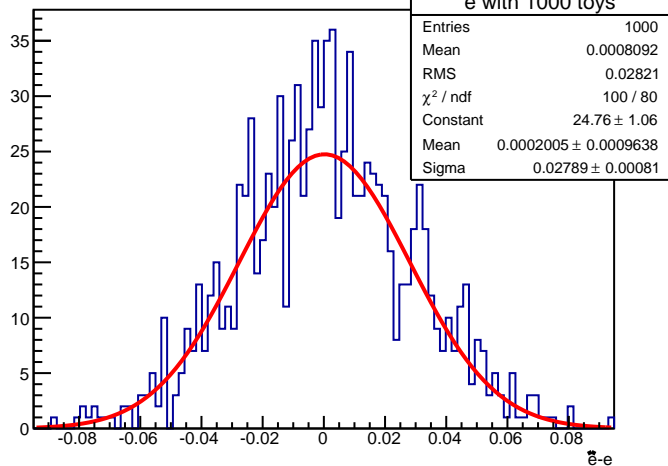
e with 1000 toys
