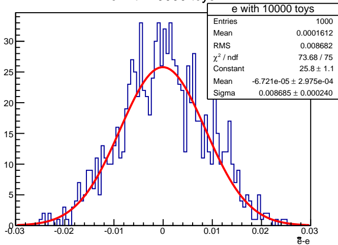
e with 10000 toys
