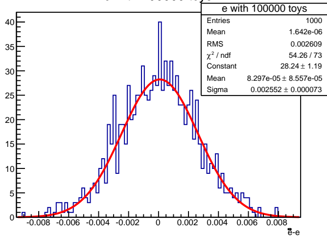
e with 100000 toys
