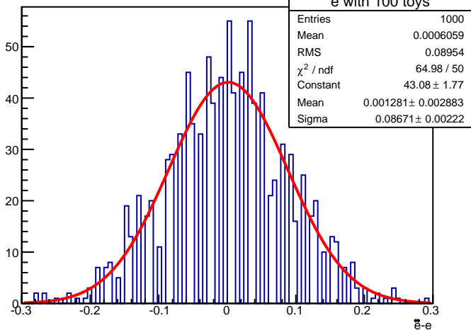
e with 100 toys
