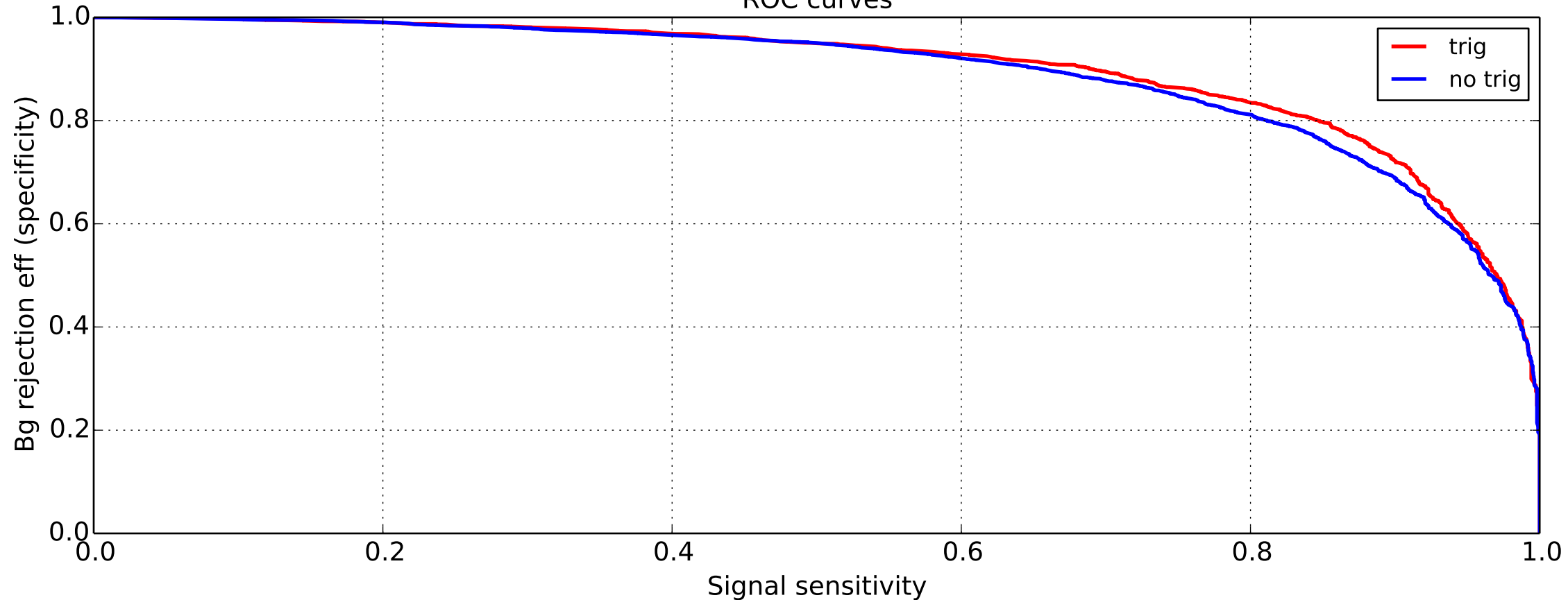
ROC curves
