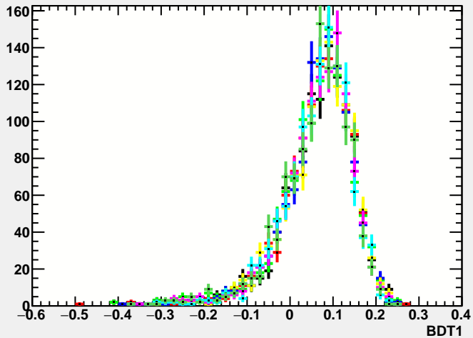
BDT1 signal 2011
