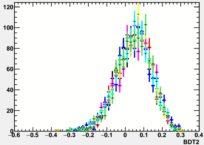
BDT2 signal 2011
