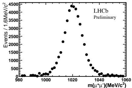
background subtracted \mu^+ \mu^- mass
