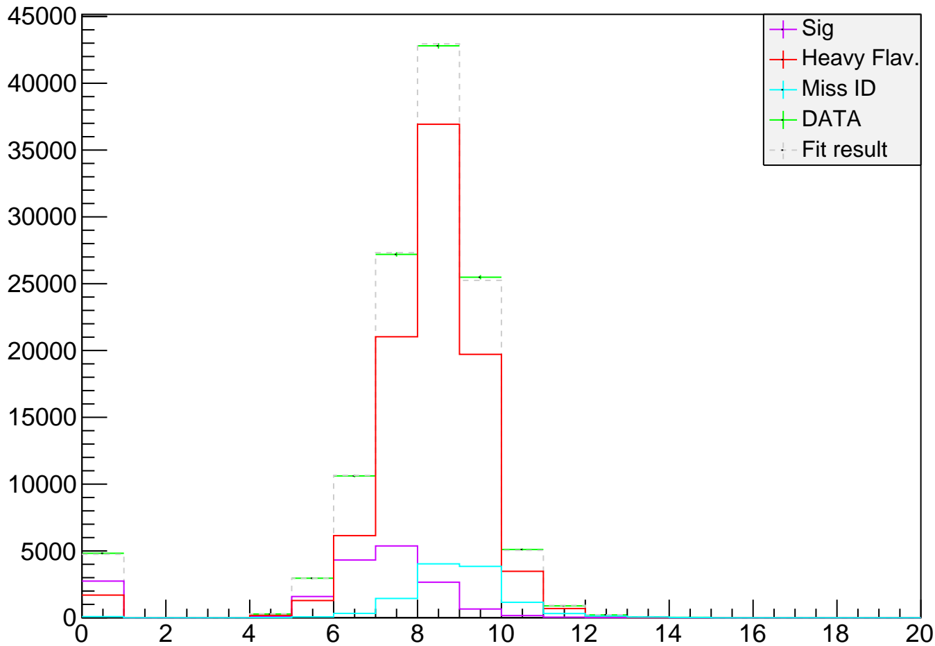
Data_12000_15000_y_bin_2.75_3
