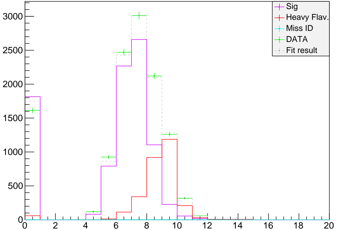
Data_30000_40000_y_bin_2_4.5
