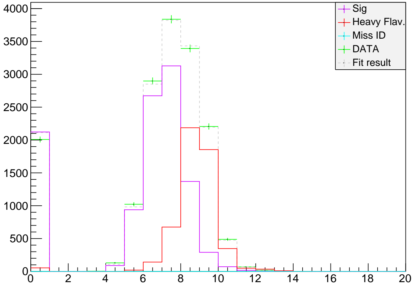
Data_25000_30000_y_bin_2_4.5
