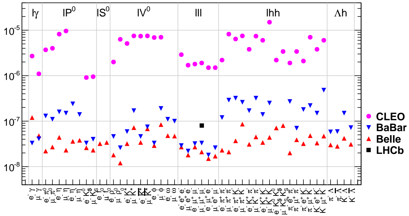
90% C.L. upper limits for LFV \tau decays
