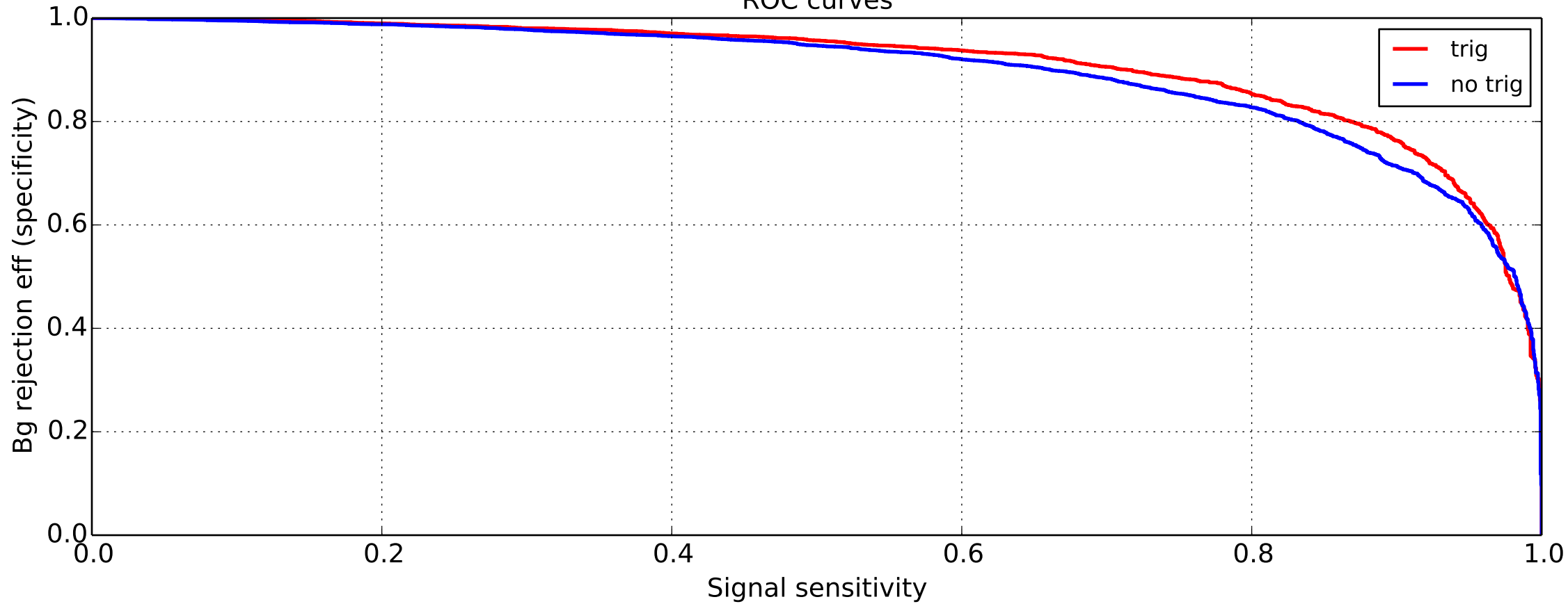
ROC curves
