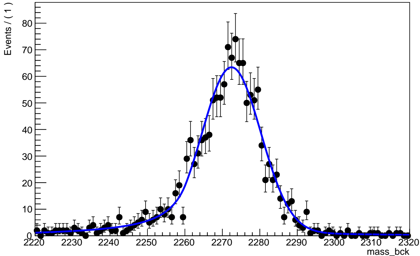
A RooPlot of "mass_bck"
