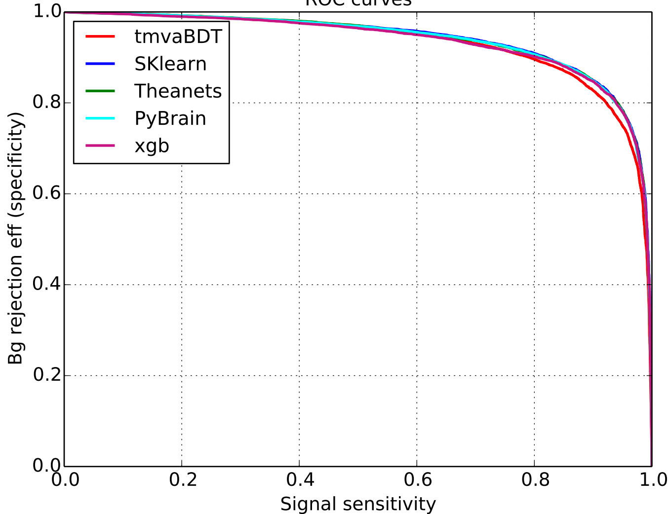
ROC curves
