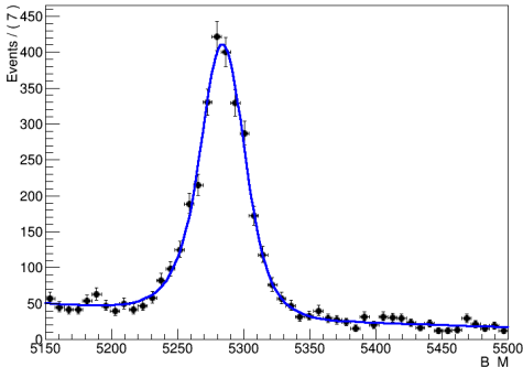
Fit to K^* J/\psi mass
