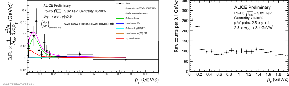
Fig. 11. Transverse momentum spectrum for J/\psi at central rapidity (left) and forward rapidity (right) in peripheral Pb–Pb collisions at \sqrt{s_{NN}} = 5.02 TeV [21].
