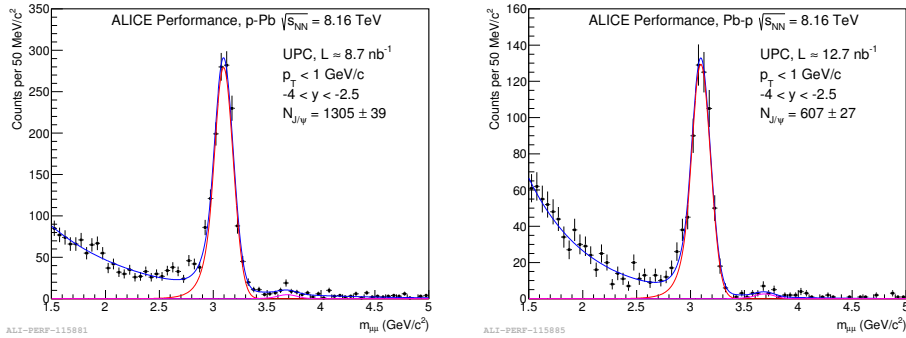
Fig. 3. Invariant mass distributions for unlike-sign dimuons with pair p_T < 1 GeV/ c and rapidity -4 < y < -2.5 in ultra-peripheral p–Pb (left) and Pb-p (right) collisions at \sqrt{s_{NN}} = 8.16 TeV, corresponding to \gamma p center-of-mass energy ranges 27 < W_{\gamma p} < 57 GeV and 700 < W_{\gamma p} < 1480 GeV respectively.
