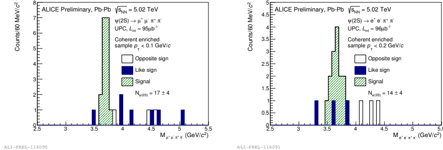
Fig. 9. Invariant mass distributions for \psi(2S) \rightarrow \mu^+\mu^-\pi^+\pi^- and \psi(2S) \rightarrow e^+e^-\pi^+\pi^- decays collected by ALICE in Pb–Pb UPC at \sqrt{s_{NN}} = 5.02 TeV.
