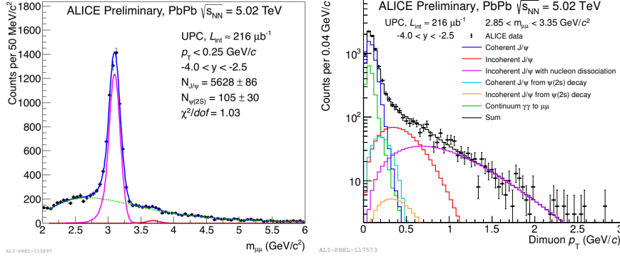
Fig. 5. Left: invariant mass distribution for unlike-sign dimuons with pair p_T < 0.25 GeV/c and rapidity -4.0 < y < -2.5 in ultra-peripheral Pb–Pb collisions at \sqrt{s_{NN}} = 5.02 TeV. Right: transverse momentum distribution for unlike-sign dimuons around J/\psi mass fitted summing six different Monte Carlo templates produced using the STARLIGHT event generator [15].
