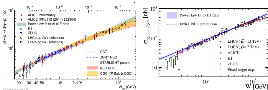
Fig. 1. Cross section of exclusive J/\psi photoproduction off protons as a function of the center-of-mass energy of the photon-proton system measured by ALICE in p–Pb collisions at \sqrt{s_{NN}} = 5.02 TeV [5] (left) and measured by LHCb in pp collisions at \sqrt{s} = 7 and \sqrt{s} = 13 TeV (right) compared to HERA data and theoretical models [6].
