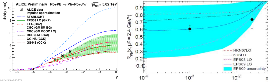
Fig. 6. Left: Measured coherent differential cross section of J/\psi photoproduction in ultra-peripheral Pb–Pb collisions at \sqrt{s_{NN}} = 5.02 TeV. Right: Gluon shadowing factor extracted from the ALICE measurements at \sqrt{s_{NN}} = 2.76 TeV [10].
