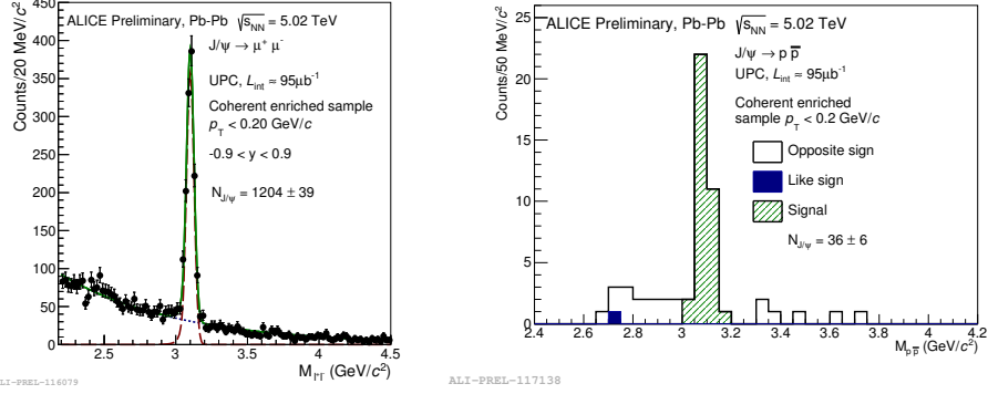
Fig. 7. Invariant mass distribution for unlike-sign dimuons (left) and diprotons (right) with pair p_T < 0.2 GeV/c and rapidity |y| < 0.9 in ultra-peripheral Pb–Pb collisions at \sqrt{s_{NN}} = 5.02 TeV.
