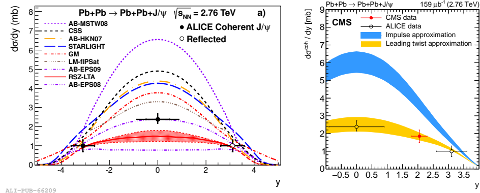
Fig. 4. Coherent J/\psi photoproduction cross section in Pb–Pb UPC at \sqrt{s_{\text{NN}}} = 2.76 TeV measured by ALICE [12] (left) and CMS [13] (right).
