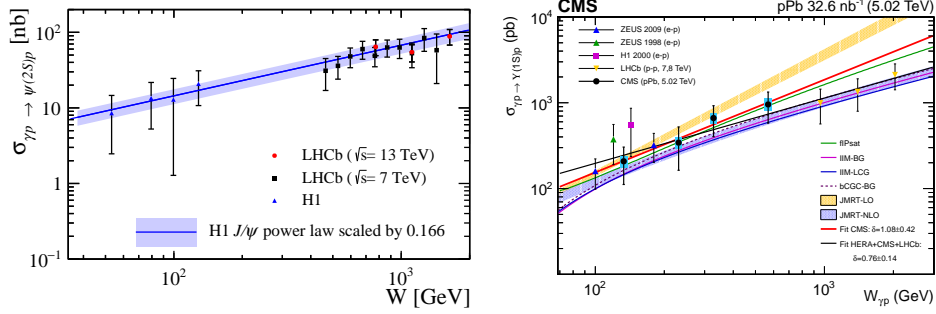
Fig. 2. Cross section of exclusive \psi(2S) (left) and \Upsilon(1S) (right) photoproduction off protons as a function of the center-of-mass energy of the photon-proton system measured by LHCb in pp collisions at \sqrt{s} = 7 and \sqrt{s} = 13 TeV [6] (left) and by CMS in p–Pb collisions at \sqrt{s_{NN}} = 5.02 TeV [7, 9].
