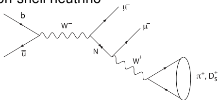
on-shell neutrino
