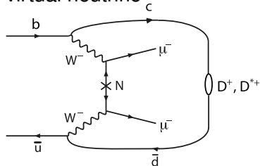
virtual neutrino
