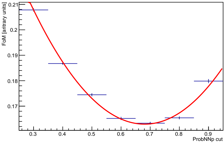
Projection ProbNNp
