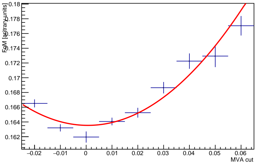
Projection MVA
