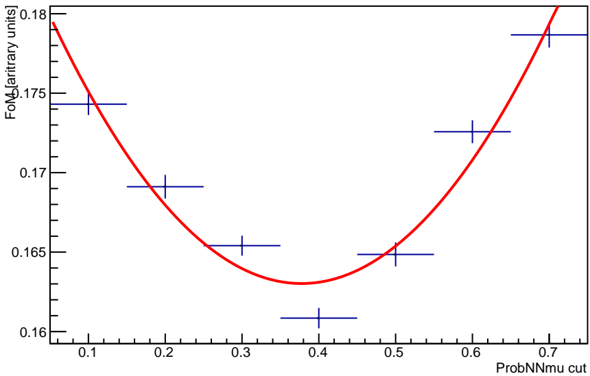
Projection ProbNNmu
