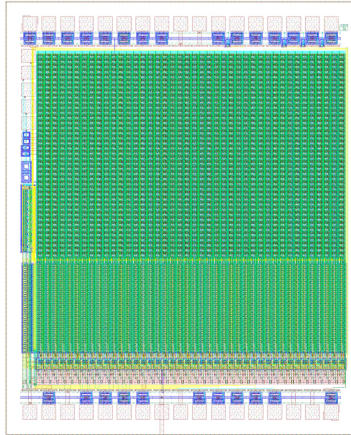
Figure 10.2: Design view of the MUXIP2 chip (actual size about 1.8 by 2.5 mm).
