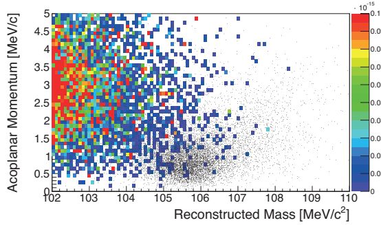
Figure 17.9: Internal conversion background (colours) and signal (black dots) in the acoplanar momentum - reconstructed mass plane for the phase IA detector configuration.
