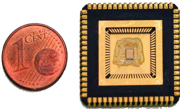
Figure 10.4: MUXIP2 sensor on ceramic carrier with one Euro-cent for scale comparison.
