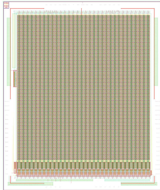
Figure 10.5: Design view of the MUXIP3 chip (actual size about 4 by 5 mm).
