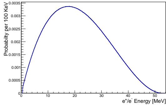
Figure 4.4: Spectrum of electrons from internal conversion decays.
