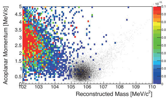
Figure 17.10: Internal conversion background (colours) and signal (black dots) in the acoplanar momentum - reconstructed mass plane for the phase IB detector configuration.
